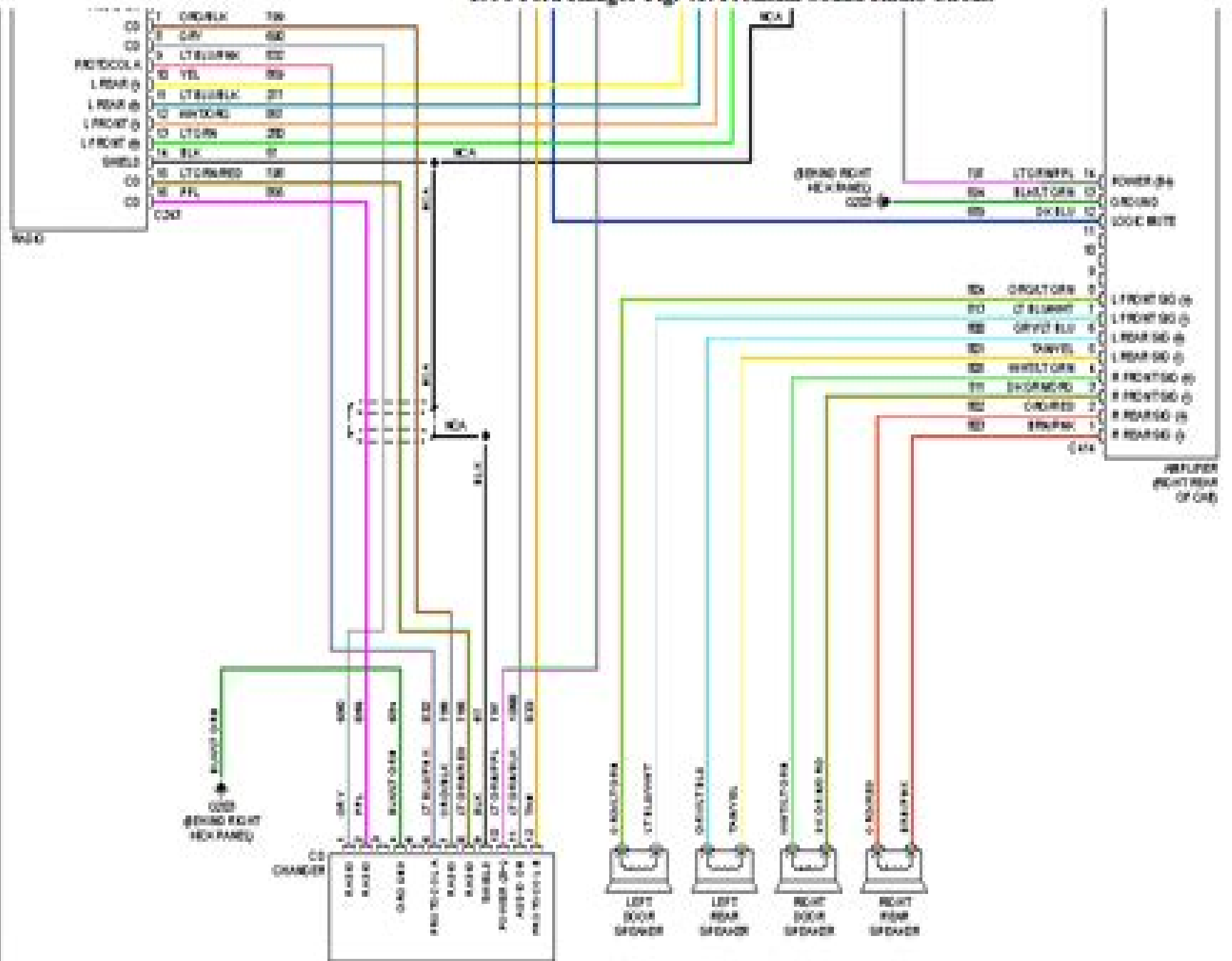
1996 Ford Ranger-Fig. 41: Premium Sound Radio Circuit
