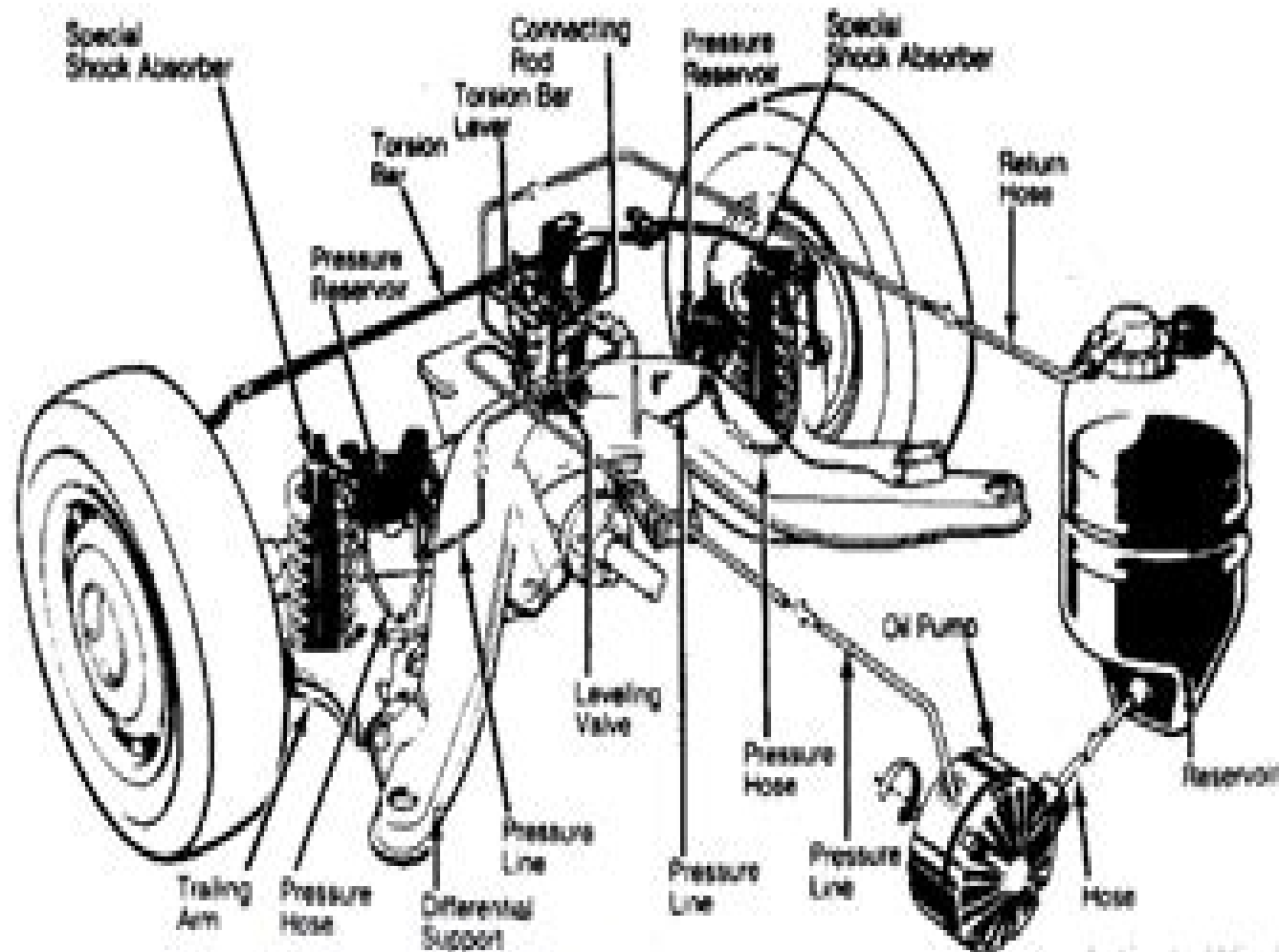
Fig. 1: Level Control Rear Suspension System (300SE, 300SEL, 300TE) Courtesy of Mercedes-Benz of North America.
