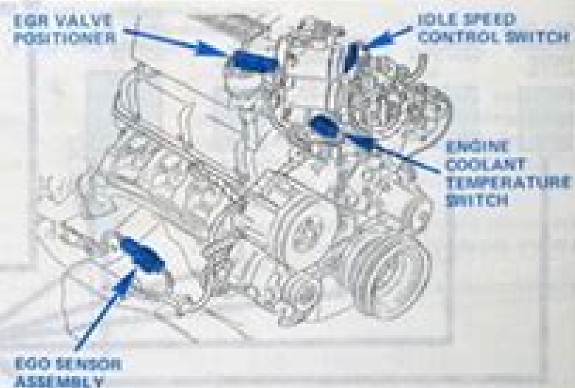
Figure 4 - RH Side of 5.0L EFI Engine
