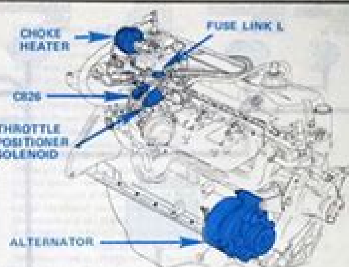
Figure 2 - RH Side of Heavy Duty 4.9L Engine
