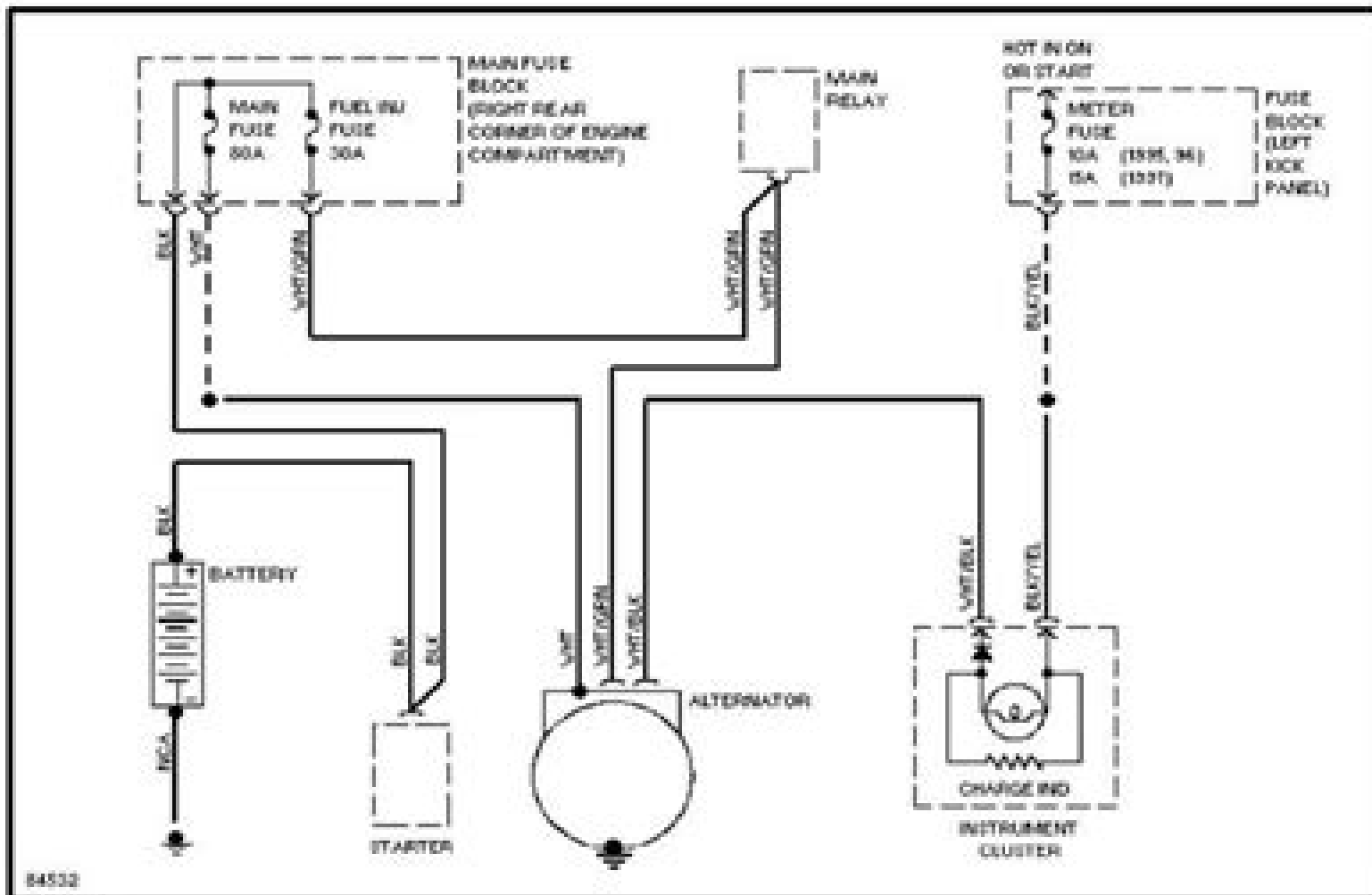
Charging Circuit
