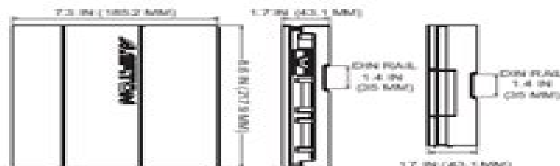
Fig. 1 ACM mounting dimensions.
