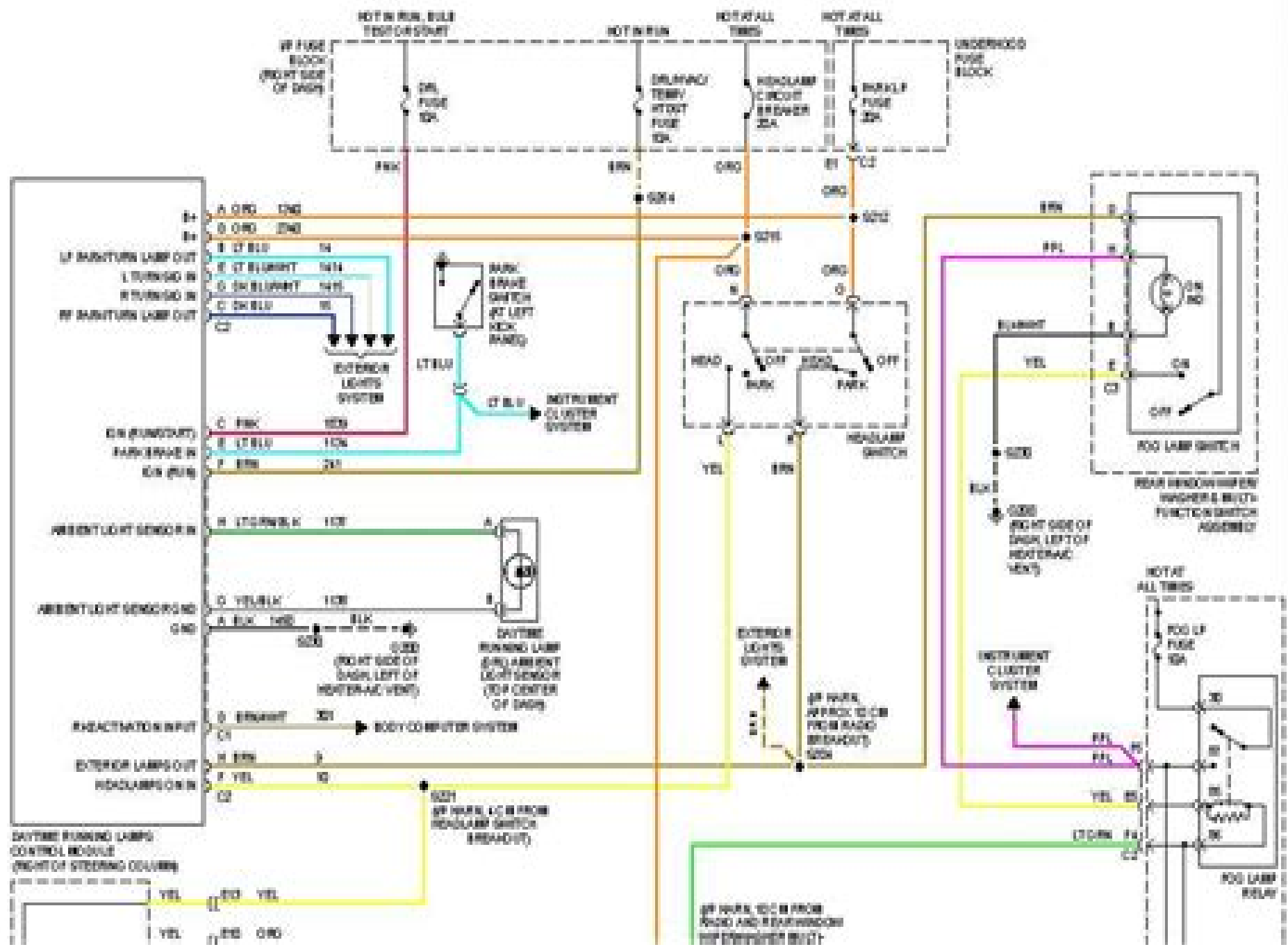
2002 Chevrolet Venture LS Fig. 26: Headlight Circuit
