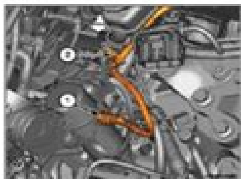
12. Disconnect the heater vacuum hose from the electric vacuum pump (1). Remove the vacuum pump (2).
