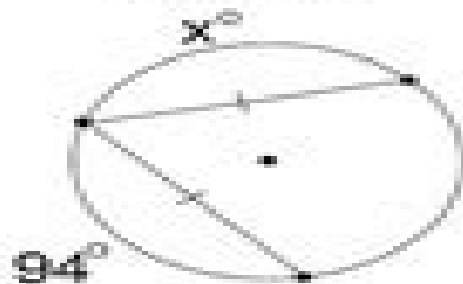
Central Angles
