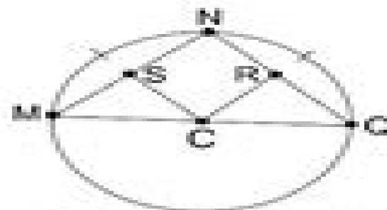
Inscribed Angles
