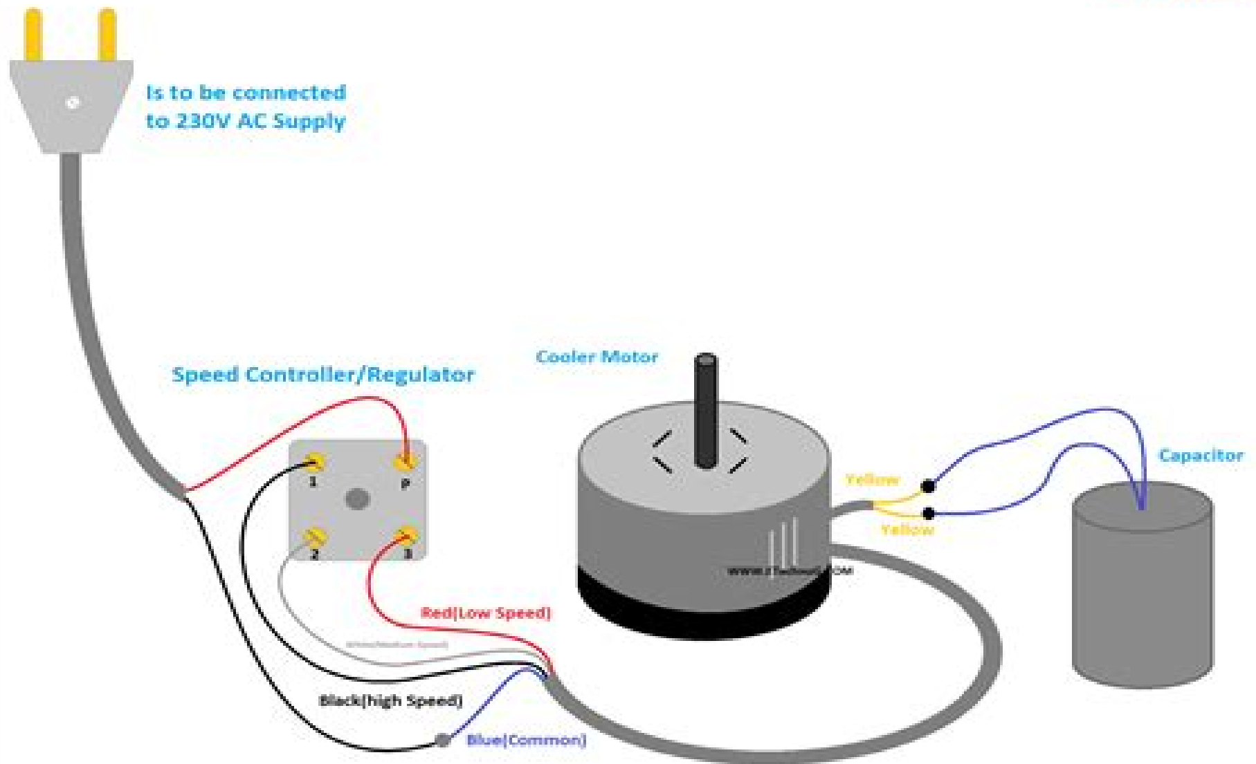
4 Wire Cooler Motor Wiring Diagram and Connection
