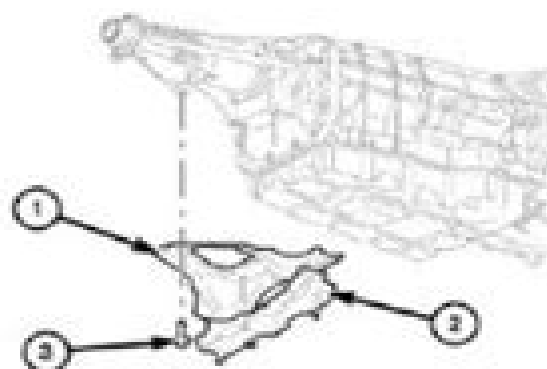
Fig. 317: Transmission Mounting Bracket, Insulator & Belt Courtesy of CHRYSLER GROUP, LLC
