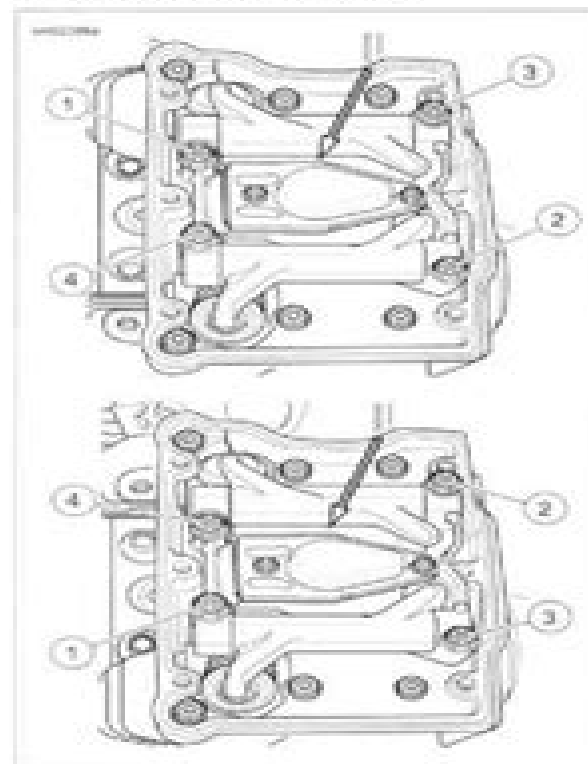
Figure 3-20. Rocker Arm Support Screw Sequence
