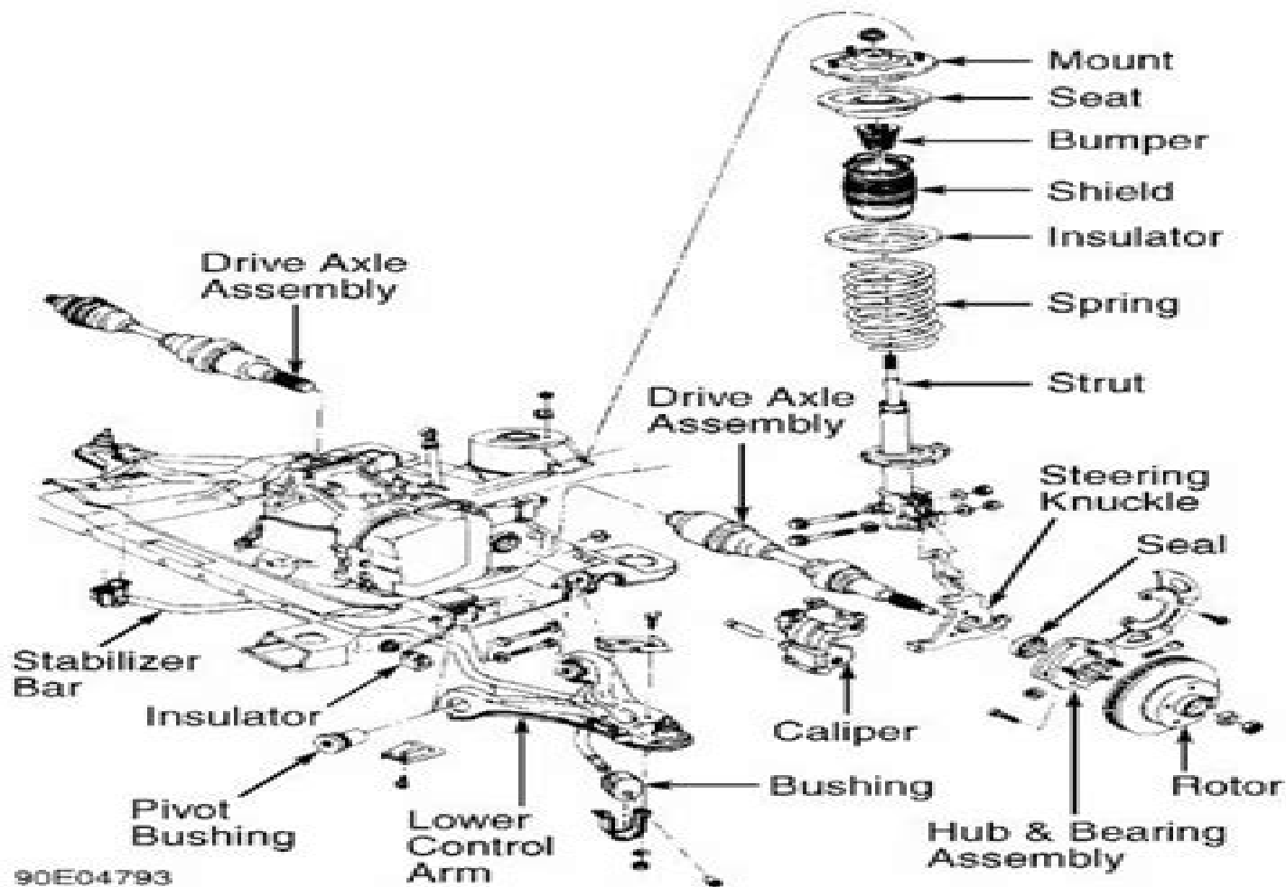
Fig. 1: Exploded View Of Front Suspension Courtesy of GENERAL MOTORS CORP.
