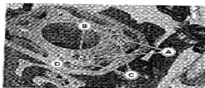
A. Exhaust Valves B. O-Rings (nothing in above fig.) C. Valve Guides D. Valve Operating Rod
