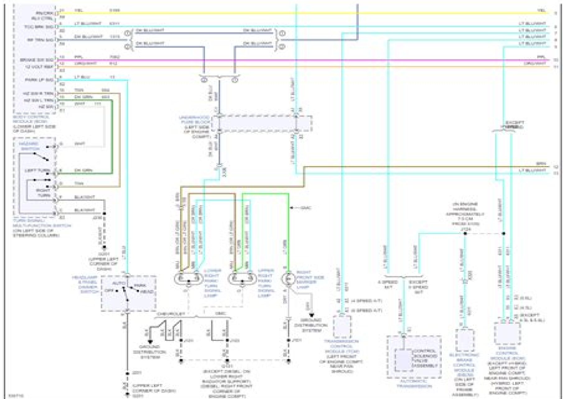
Fig 2: Exterior Lamps Circuit (1 of 3)
