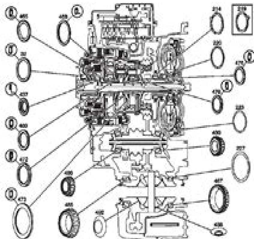
Fig. 14: Identifying Bushing & Bearing Locations
