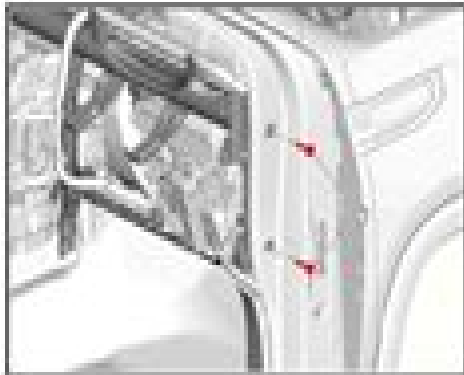
Instrument Panel Tie Bar Bolt (1) & Floor Side Door - Install and tighten [2x] 22 N.m (16 ft.lb)
