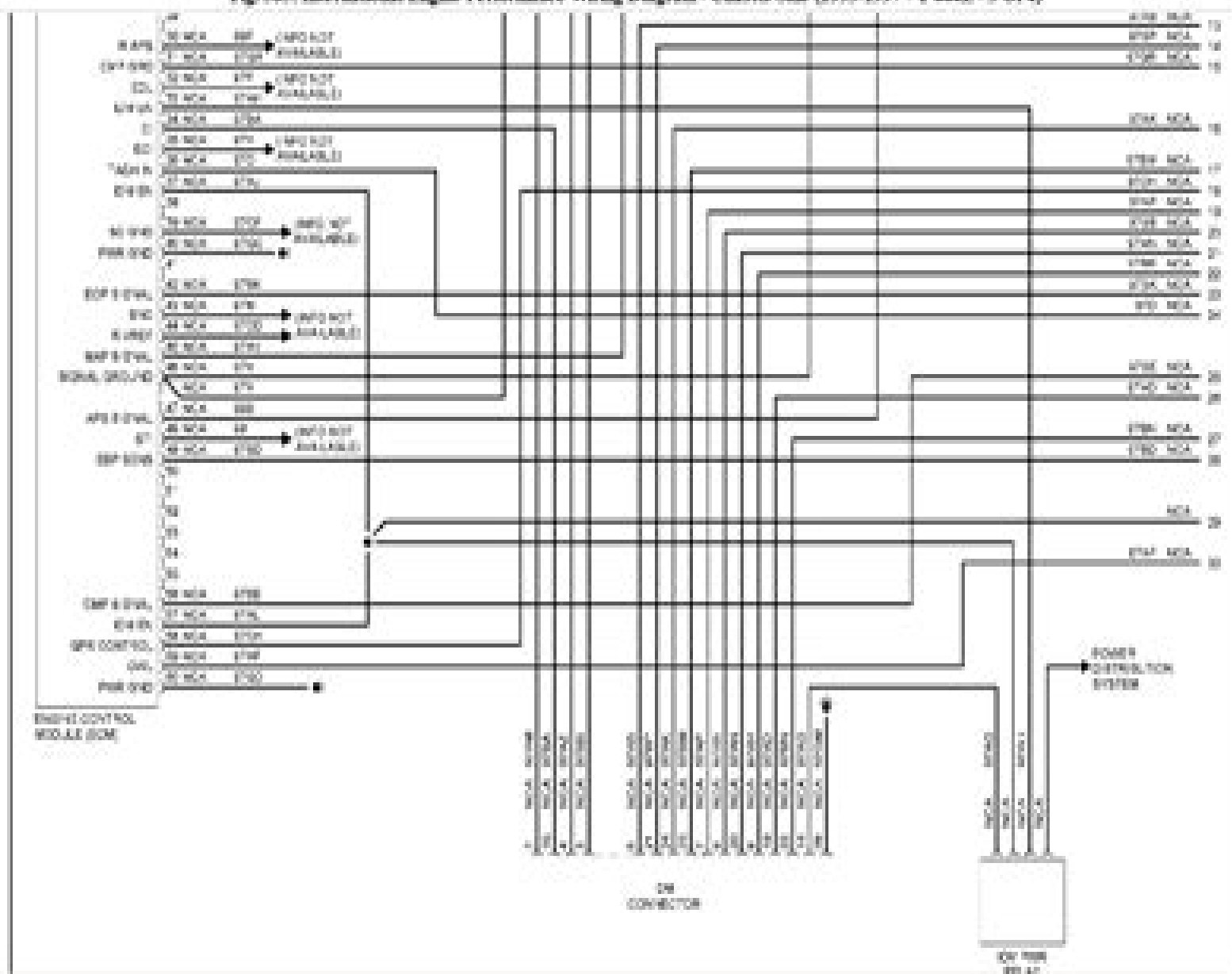
Fig. 565: International Engine Performance Wiring Diagram - Chassis Side (1993-1997 - T 444E - 3 Of 4)
