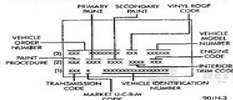
Fig. 3 Body Code Plate BODY CODE RECORDING
