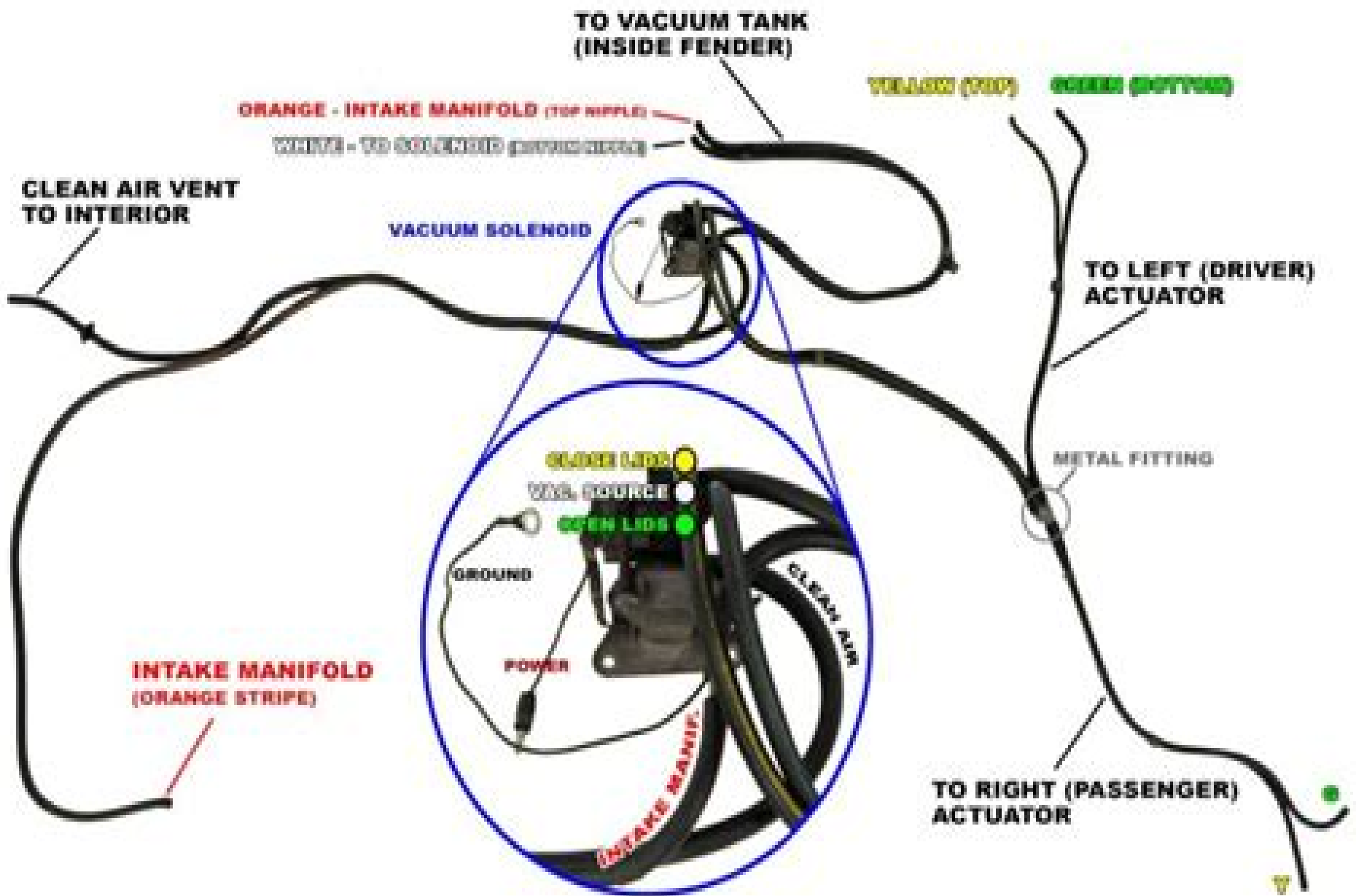
EARLY 1967 MERCURY COUGAR HEADLIGHT VACUUM HOSE CONFIGURATION
