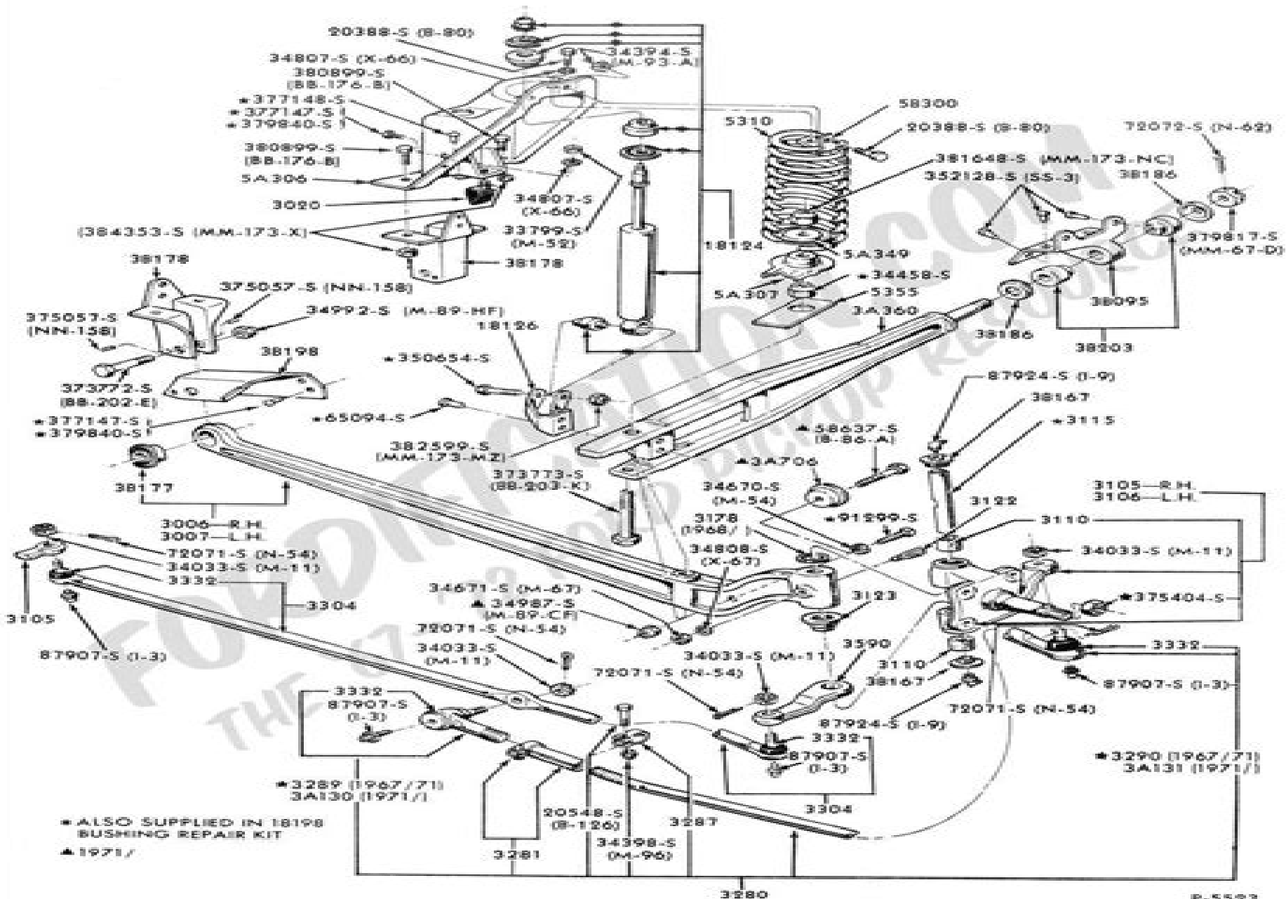
FRONT AXLE (TWIN "I" BEAM) & FRONT SUSPENSION (3.8M) 1967/69 F350
