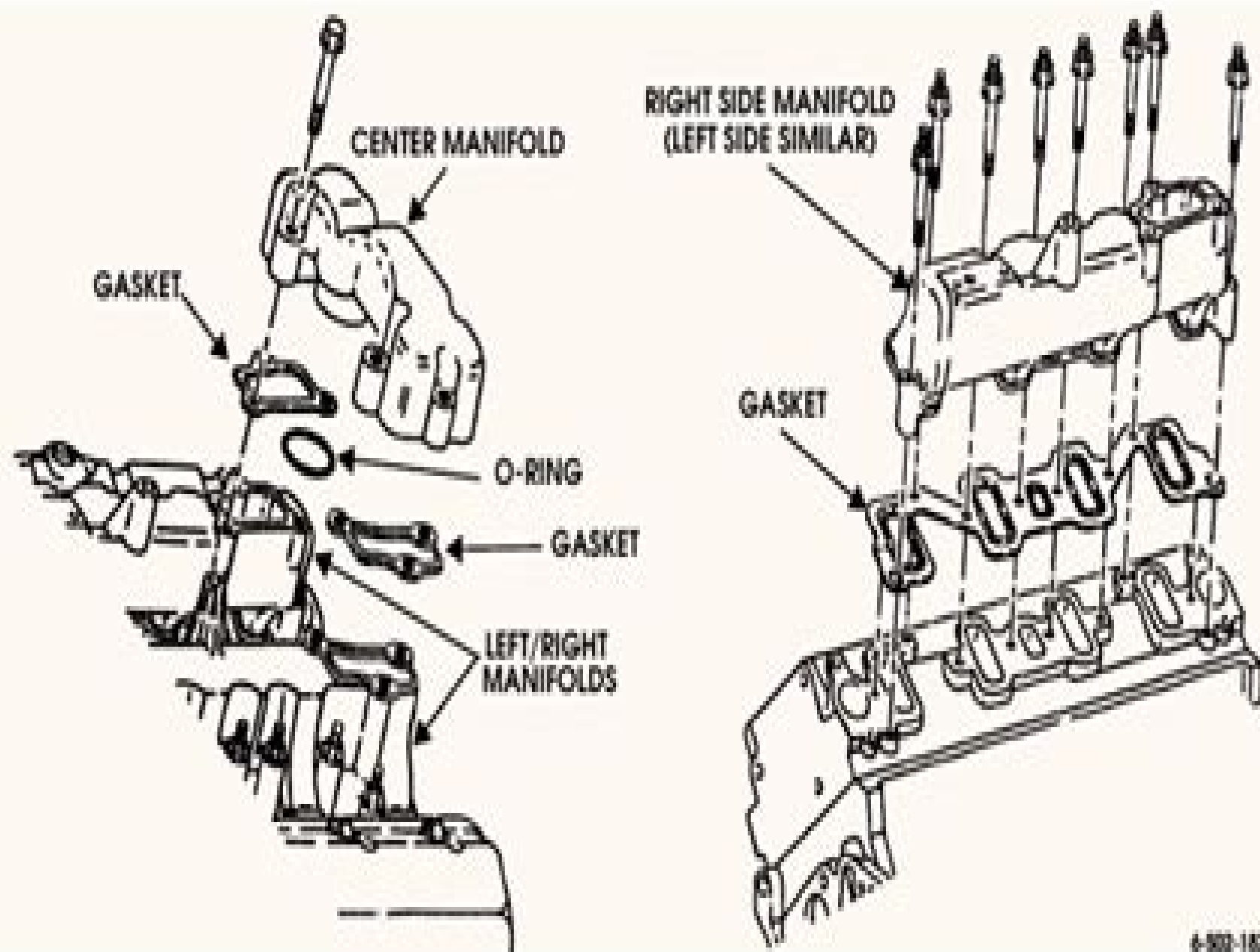
Figure 2-49: Intake Manifold Attachment
