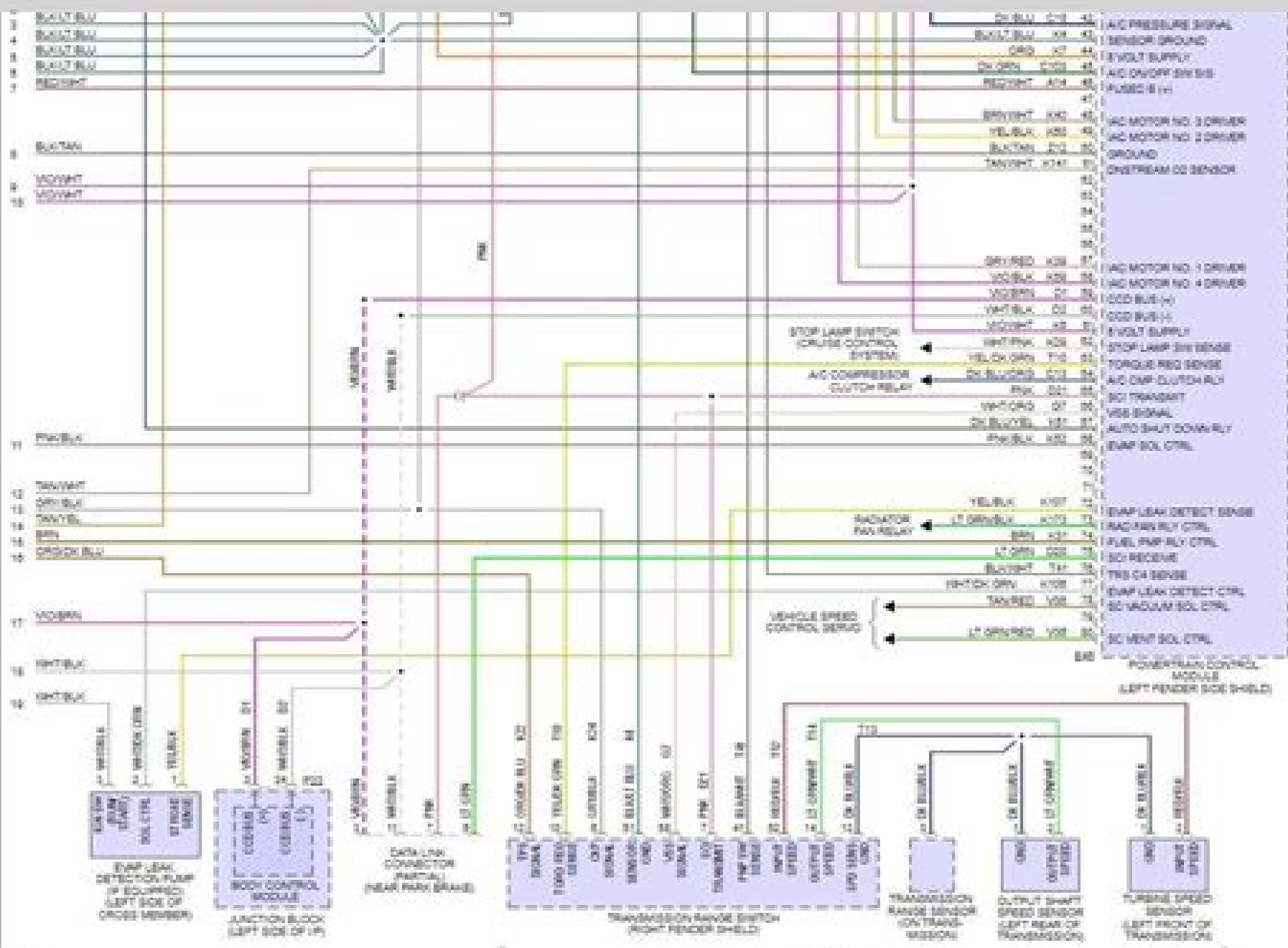
Fig 6-3.3L Engine Performance Circuits (3 of 3)
