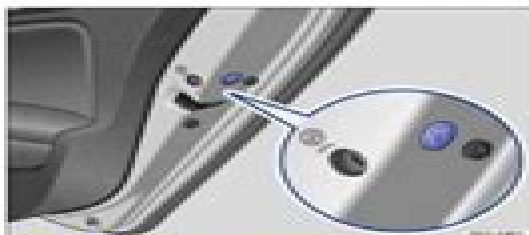
Fig. 150 On the front side of the right rear door: Emergency lock, covered by a rubber seal.
