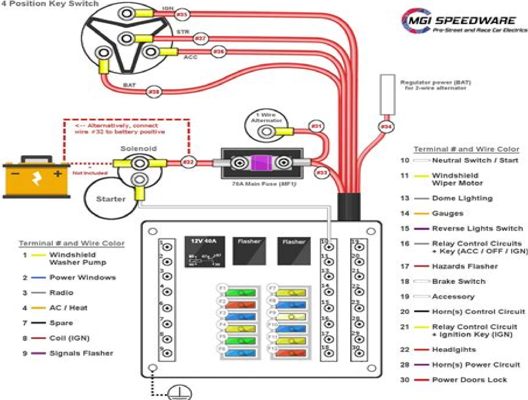
AFP12 Fuse Panel
