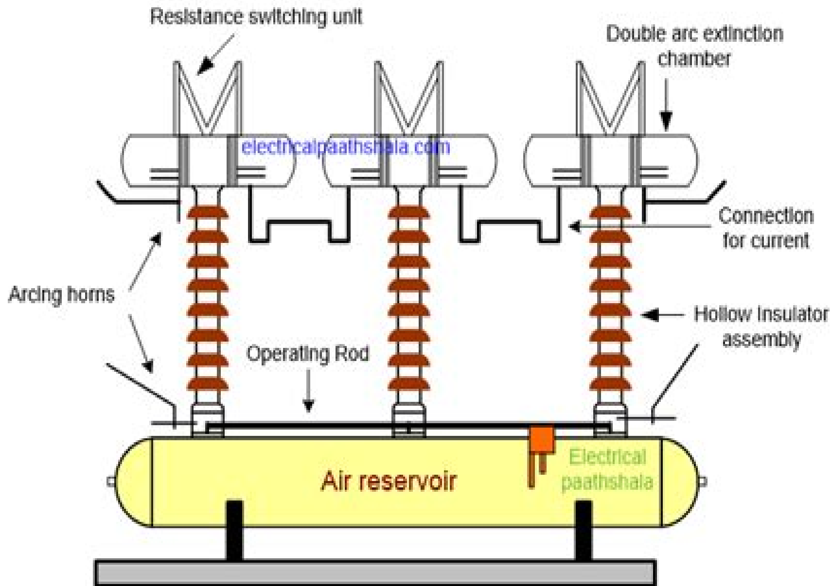
Air blast circuit breaker
