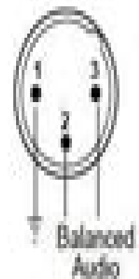
C 0377 3 Pin XLR Wiring Diagram
