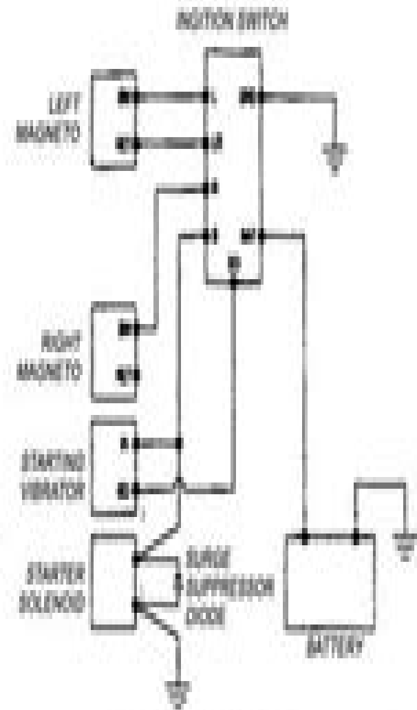
WIRING DIAGRAM FOR IGNITION SWITCH WITH STRAT POSITION & 2-TERMINAL STARTING VIBRATOR
