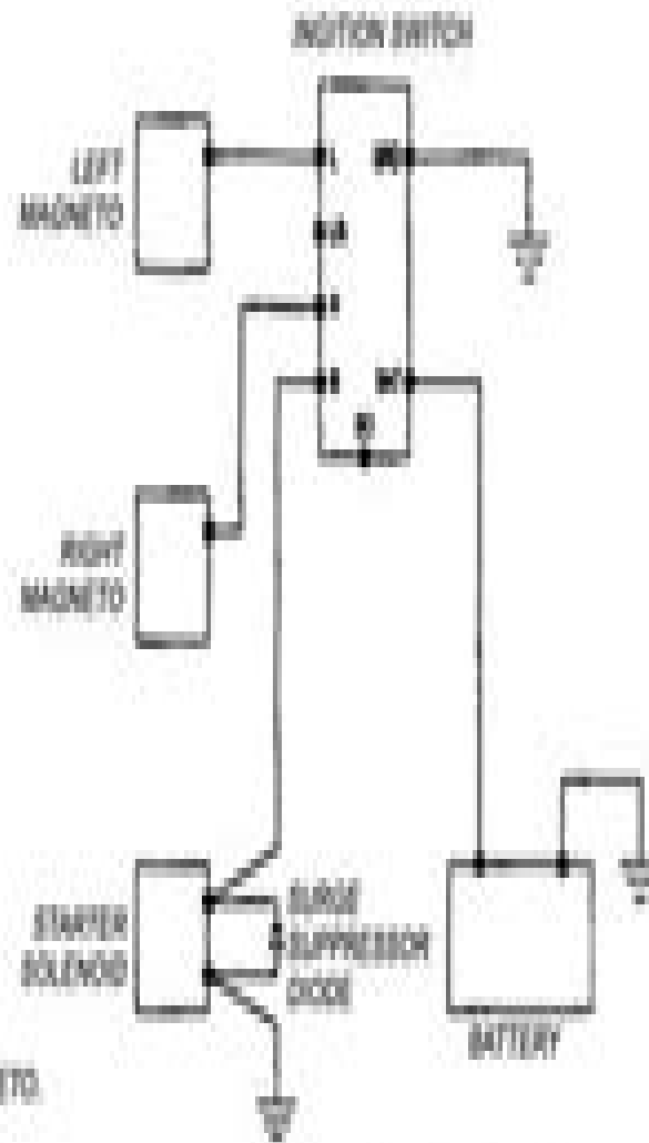
WIRING DIAGRAM FOR IGNITION SWITCH WITH STRAT DIAGRAM
