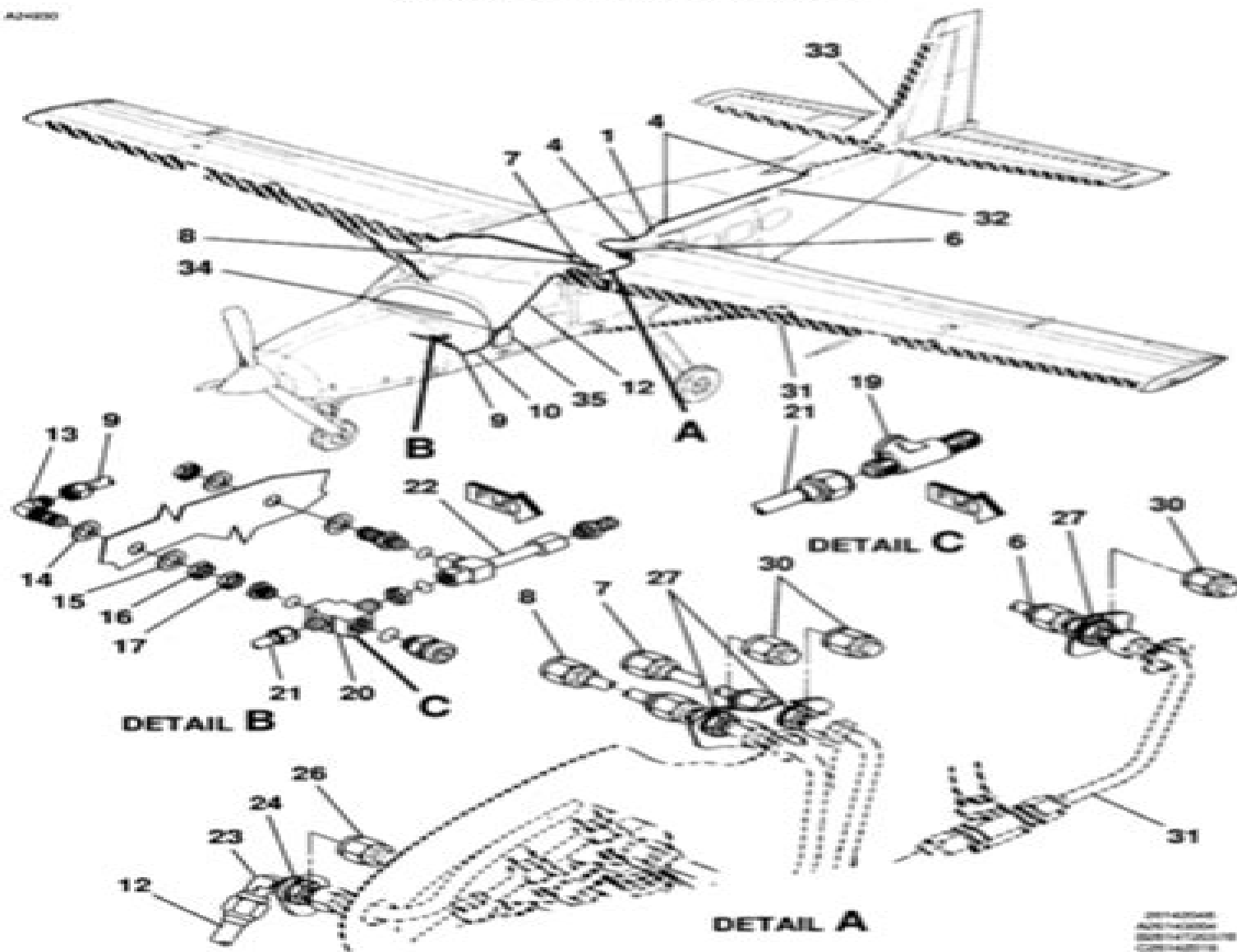
DEICE SYSTEM FIGURE 01 (SHEET 1)
