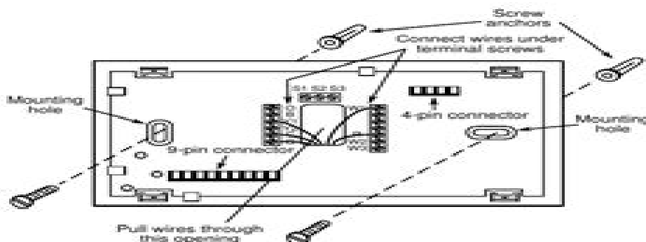
Figure 3. Subbase
