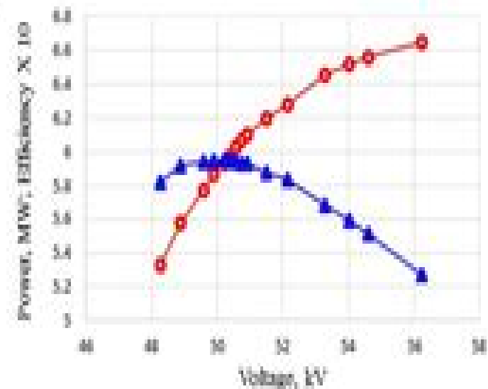
Figure 5: The efficiency (triangular) and RF power production (circle) in saturation at 3.003 GHz as functions of high voltage.
