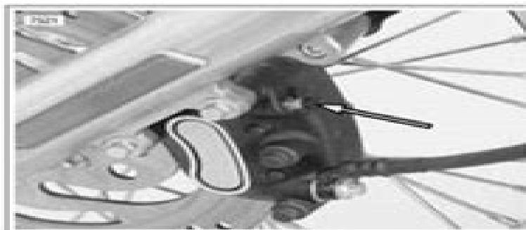
Figure 1-14. Front Brake Bleeder Valve
