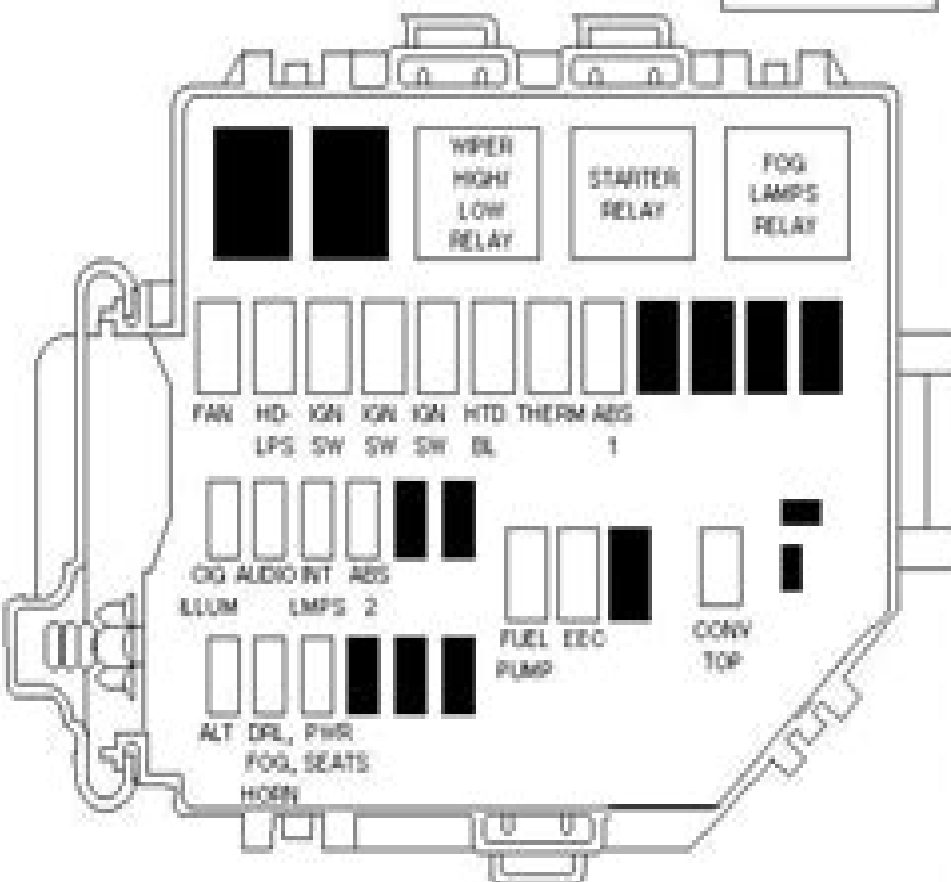
MAXI-FUSE CARTRIDGE TOP VIEW
