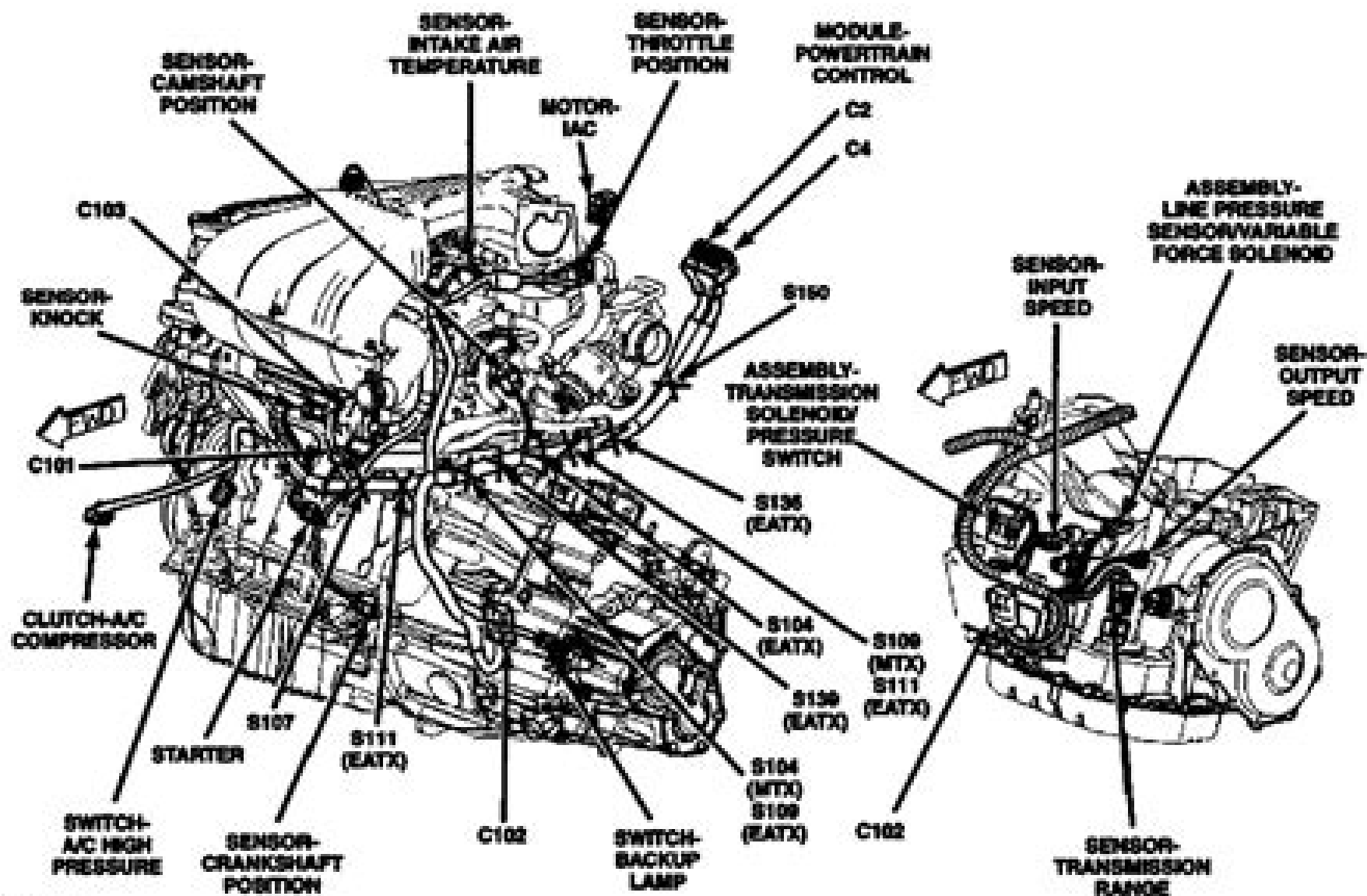
Fig 1: Engine/Transmission Assembly (Turbo)
