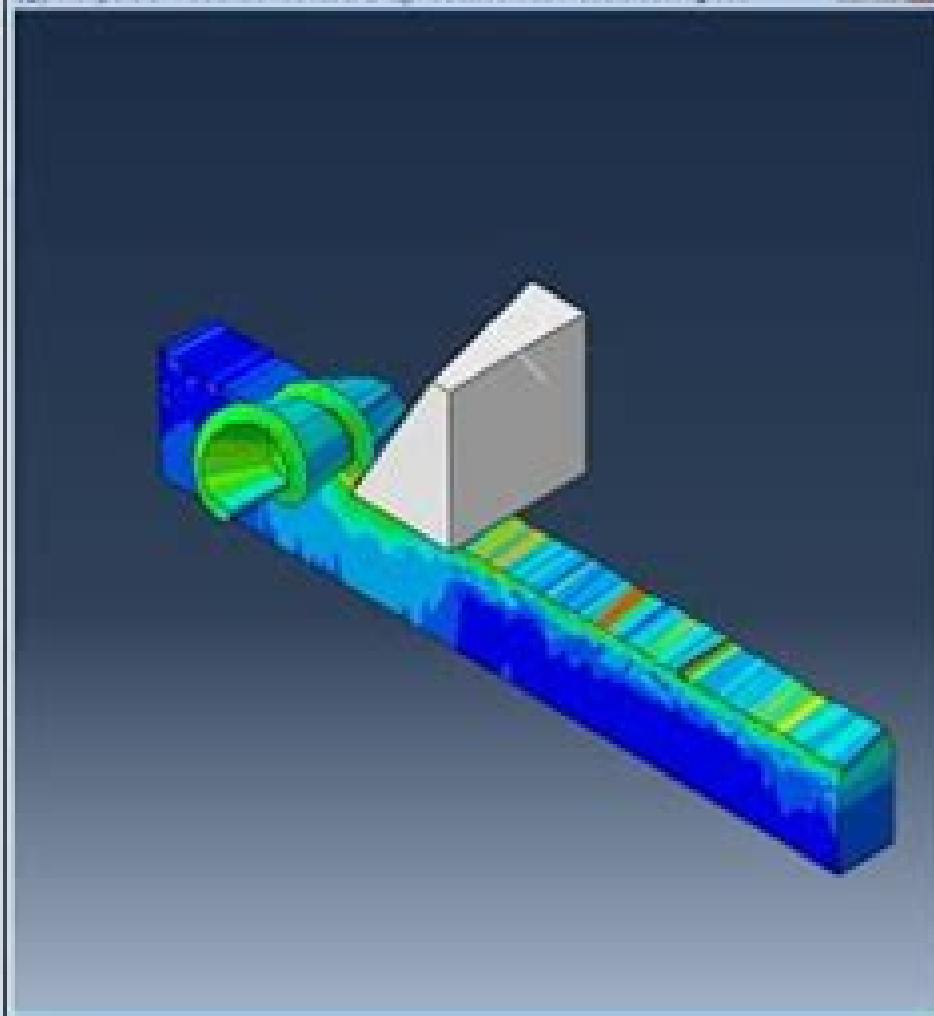
Viewport 2 009: C:\YouTube\CAE_Models\Johnson-Cook\Cutting.off
