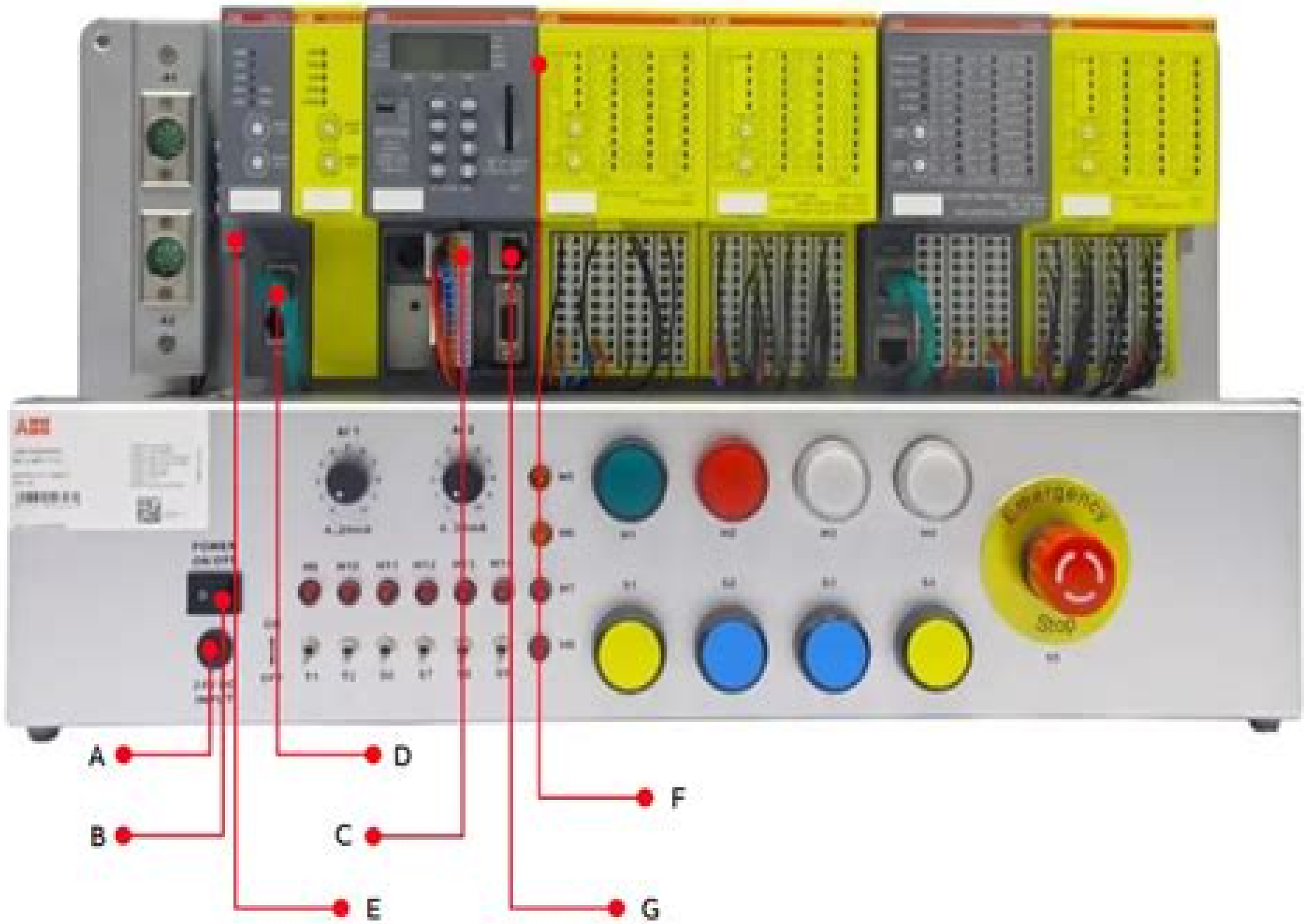
Figure 1: Front view of TA514-SAFETY training case
