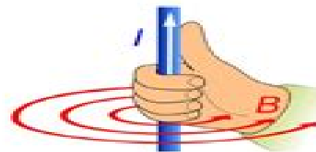
Right-hand rule
