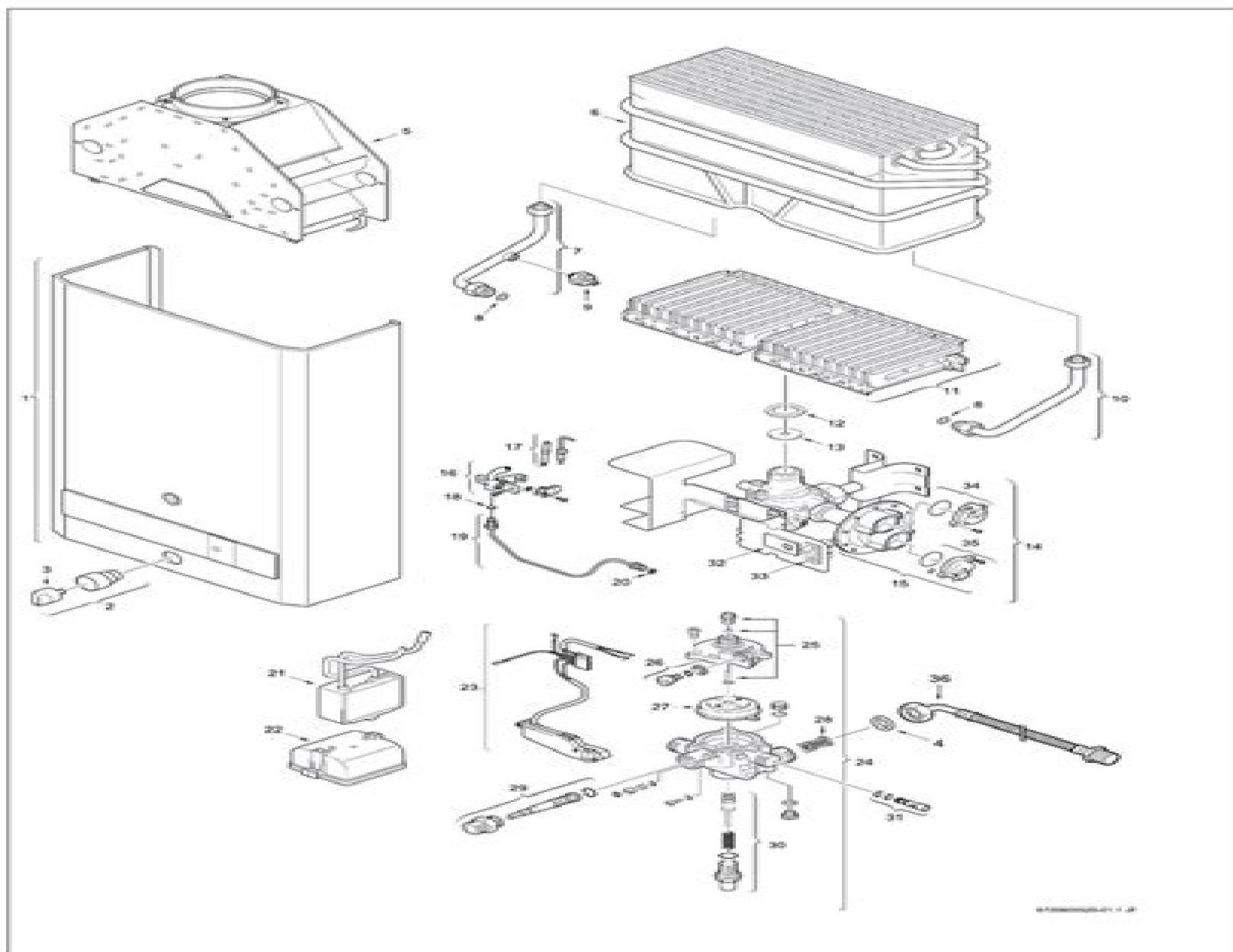
Fig. 15 - INTERIOR COMPONENTS DIAGRAM AND PARTS LIST
