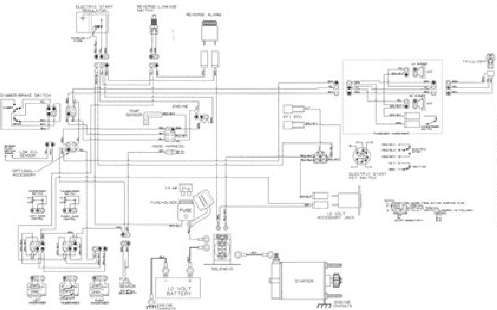
WIRING DIAGRAM (MAIN HARNESS-Partners 550 EFI)
