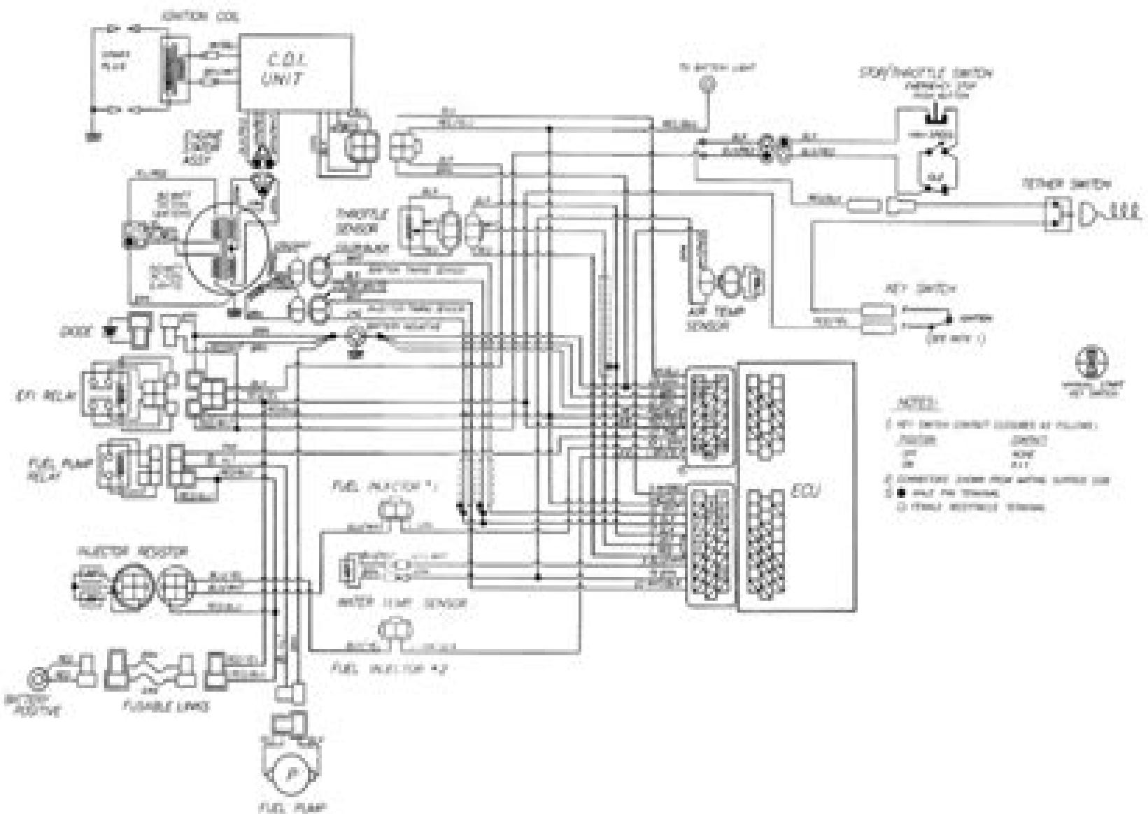
Wiring Diagram (Engine Ignition)
