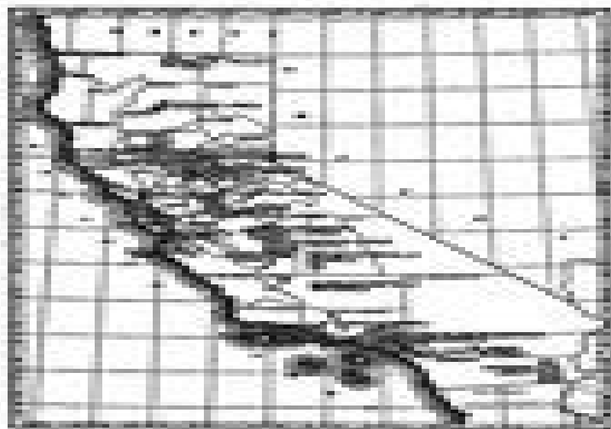
FIG. 1.—Location map showing position of the Madera area, California.
