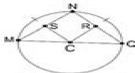
Inscribed Angles
