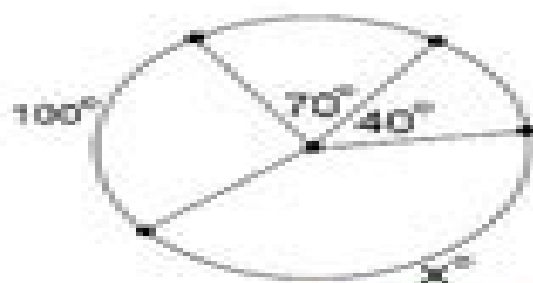
Central Angles
