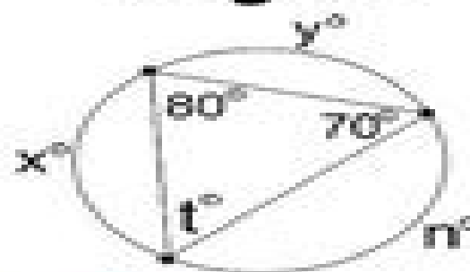
Inscribed Angles
