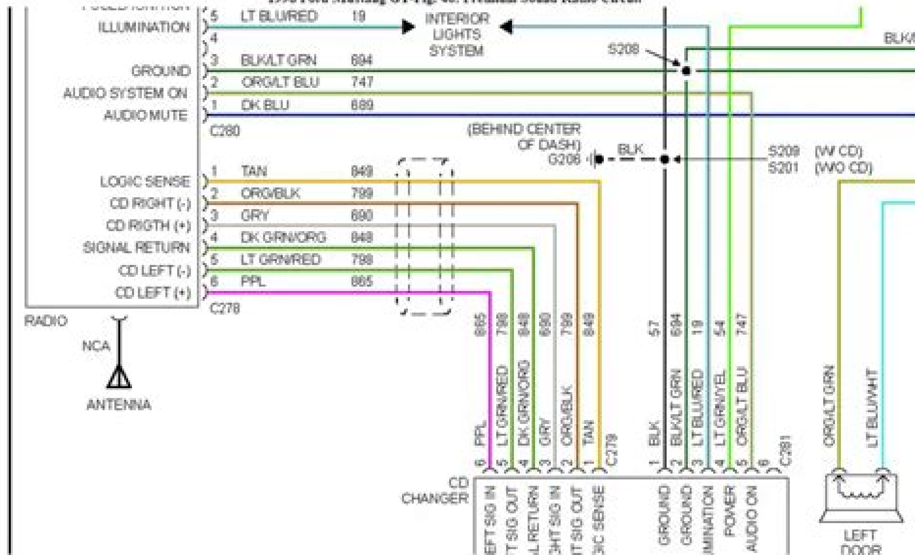
1998 Ford Mustang GT-Fig. 46: Premium Sound Radio Circuit
