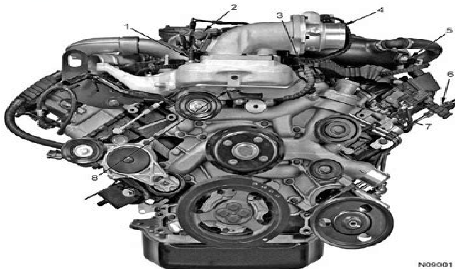
Figure 150 Sensor locations – front (typical)
