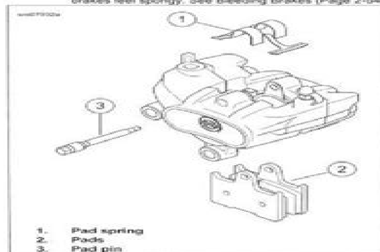
Figure 1-25. Rear Brake Pads
