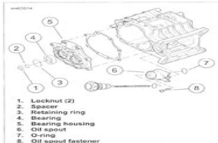
Figure 6-35. Bearing Housing Bearings
