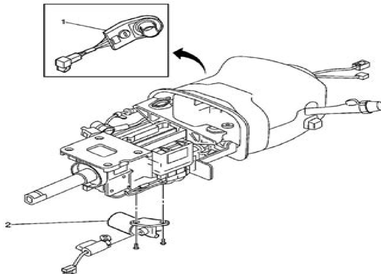
Fig. 5: Identifying Steering Wheel Theft Deterrent Lock & Tilt Actuator At LR of Steering Column Courtesy of GENERAL MOTORS CORP.
