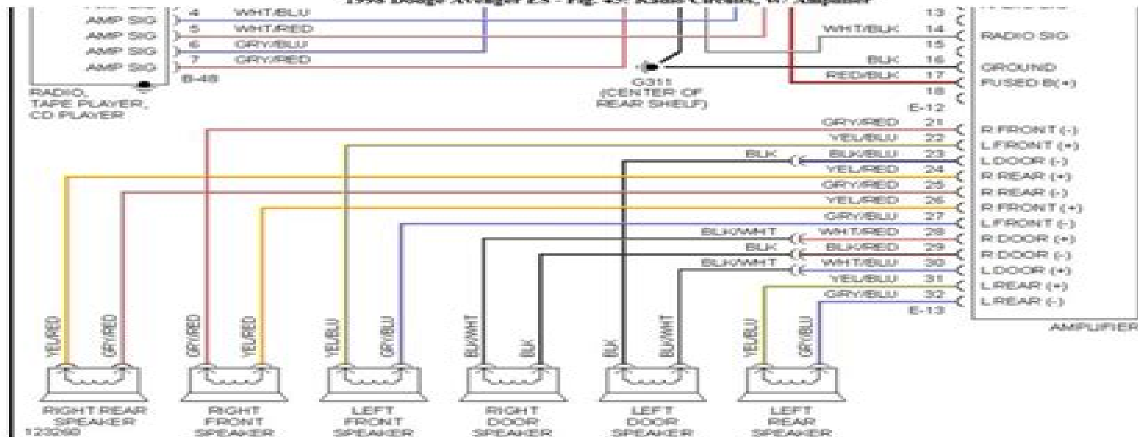
1998 Dodge Avenger ES - Fig. 45: Radio Circuits, W/ Amplifier
