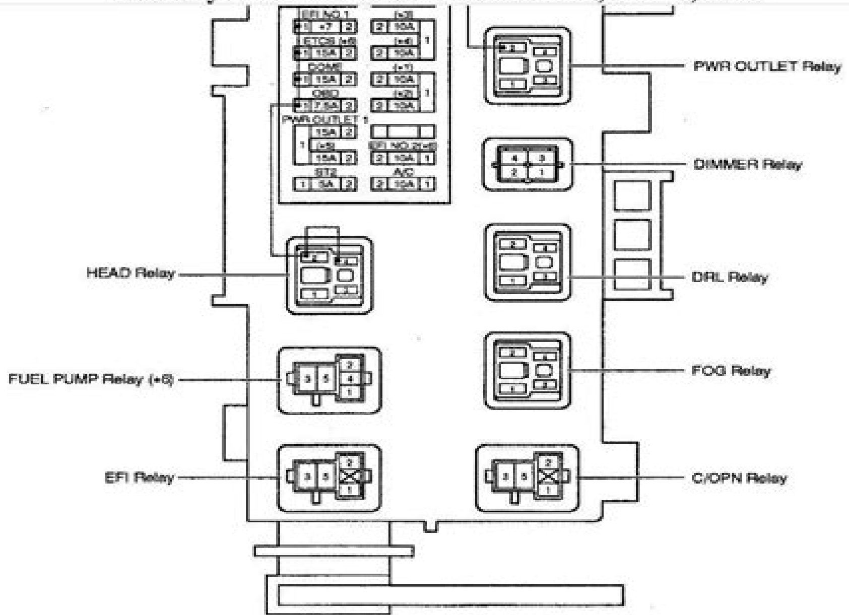
Fig. 3: Identifying Engine Compartment Relay Block Fuse Components Courtesy of TOYOTA MOTOR SALES, U.S.A., INC.
