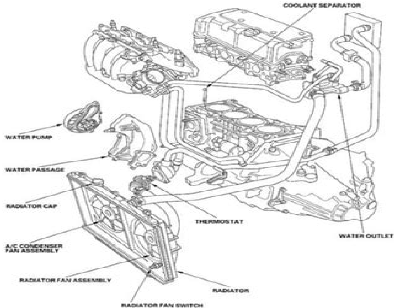
Fig. 1: Locating Cooling System Components
