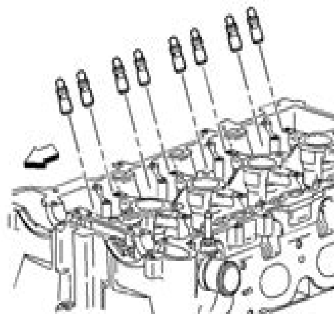
Fig. 17B: View Of Hydraulic Element Lash Adjusters Courtesy of GENERAL MOTORS CORP.
